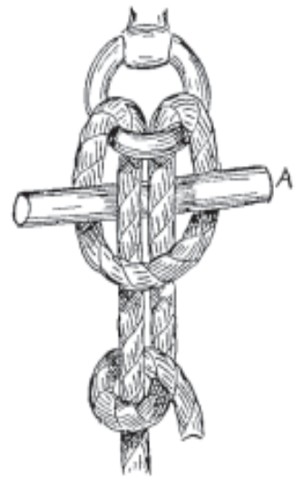
FIG. 30.—Lark's head with toggle (A).
