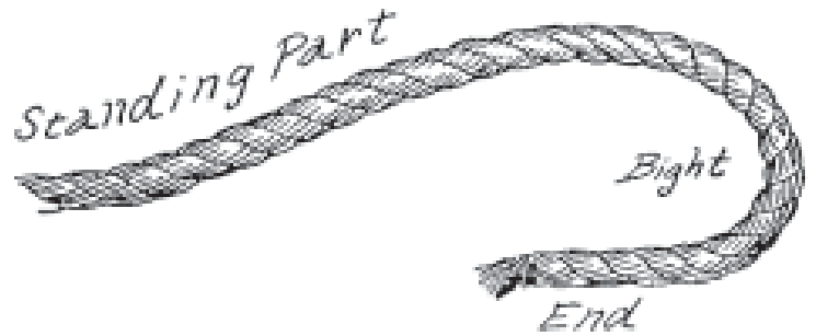
FIG. 3.—Parts of rope.
