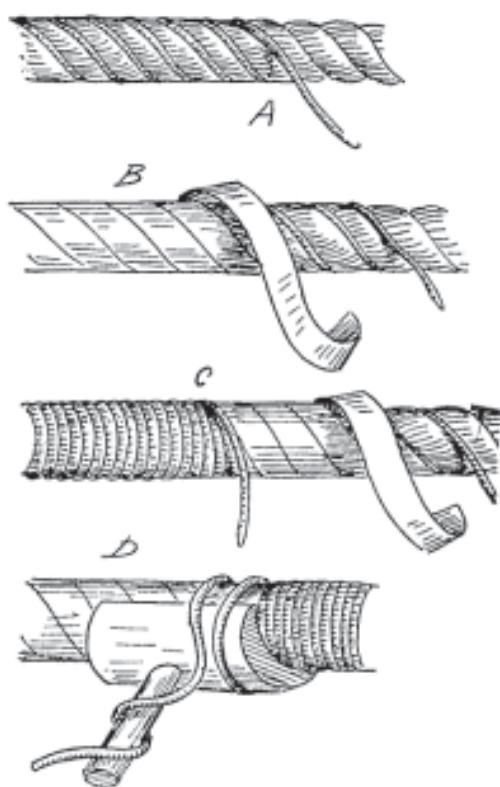
FIG. 138.—Worming, parcelling, and serving.
