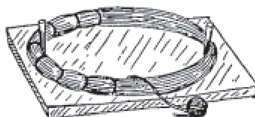
FIG. 89.—Seizing a selvagee strap.
