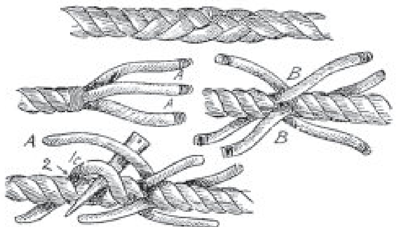
FIG. 106.—Short splice.
