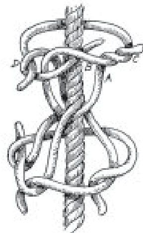
FIG. 119.—French shroud knot (making).
