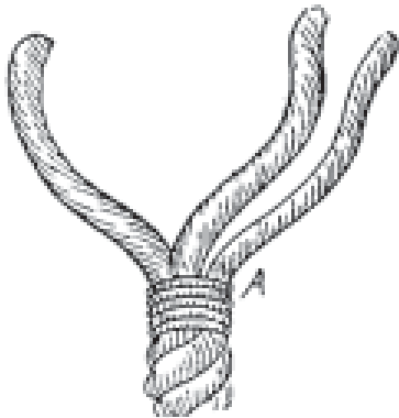
FIG. 104.—Ending rope.
