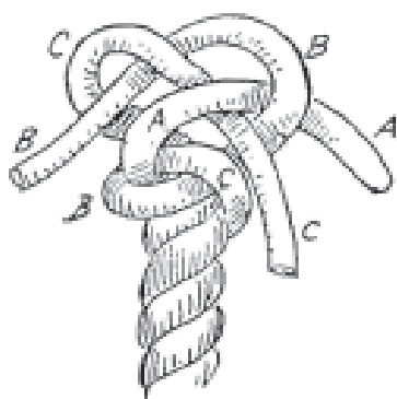
FIG. 124.—Wall crowned (making).
