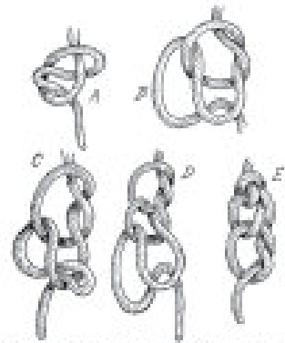
FIG. 70.—Single plait or monkey chain (making).
