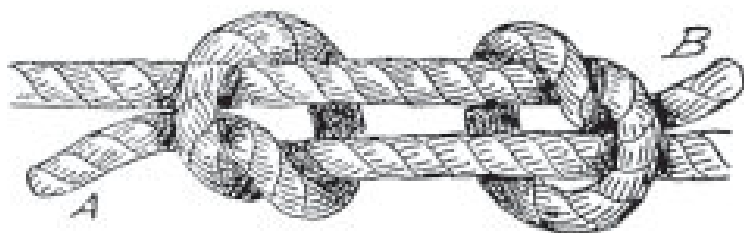
FIG. 17.—Fisherman's knot (making).
