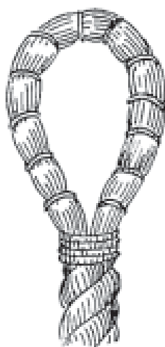
FIG. 90 B.—Flemish eye (complete).
